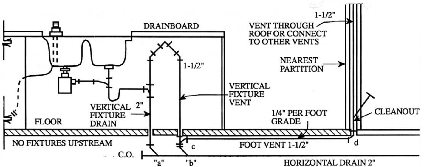
A, B AND C ARE Y-BRANCH FITTINGS
