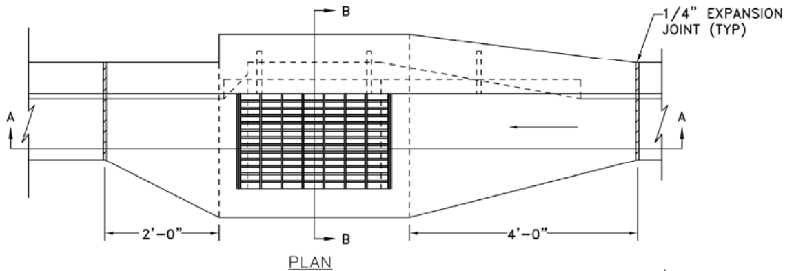
TYPE I GUTTER – LONGITUDINAL STREET GRADE LESS THAN 5%
