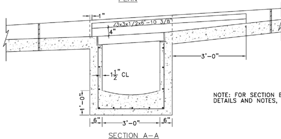
TYPE II GUTTER – LONGITUDINAL STREET GRADE 5% AND GREATER
