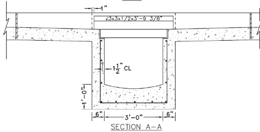
TYPE I GUTTER – LONGITUDINAL STREET GRADE LESS THAN 5%
